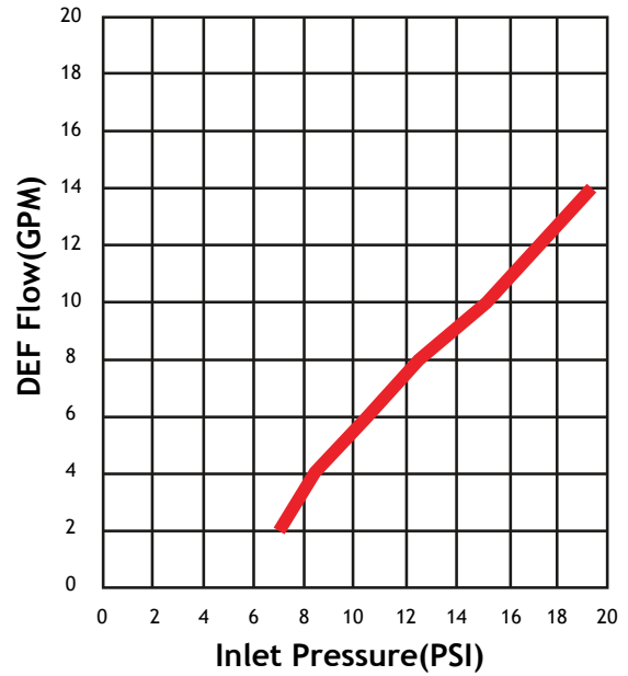
POLY DEF NOZZLE AVERAGE BACK PRESSURE PERFORMANCE VERIFICATION
