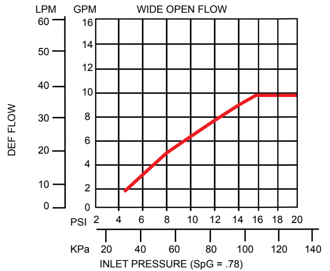
SST DEF NOZZLE AVERAGE BACK PRESSURE PERFORMANCE VERIFICATION
