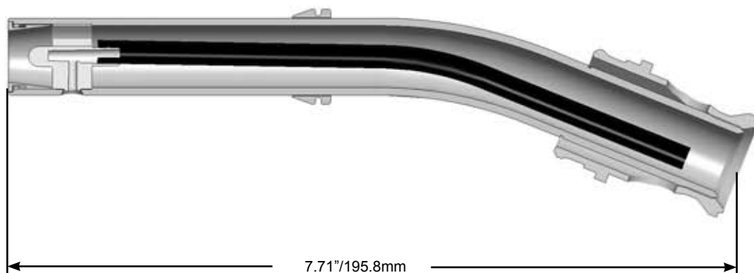
Vacuum Assist Vapor Recovery
