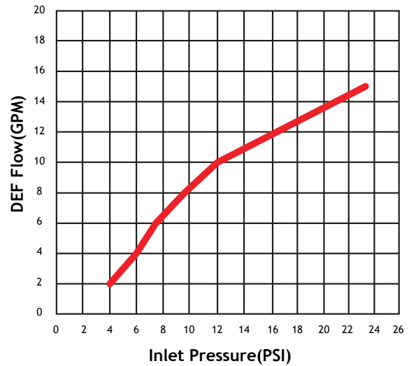
X DEF NOZZLE AVERAGE BACK PRESSURE PERFORMANCE VERIFICATION
